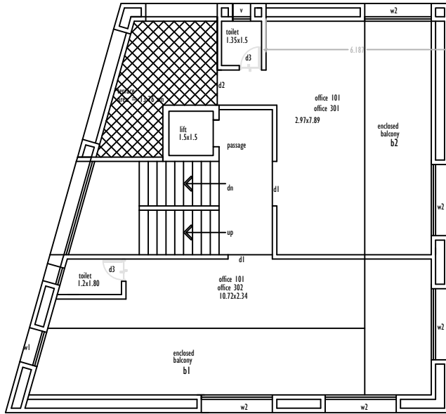
typical first and third floor plan
